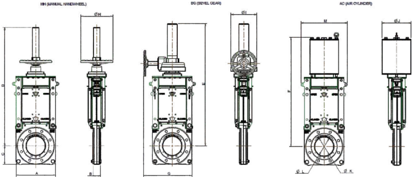
Dimensions (mm) and Weights (kg)
